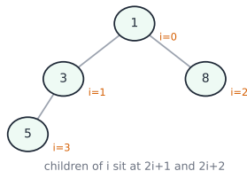
min-heap array [1, 3, 8, 5]
