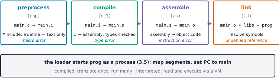
source to process: four stages, four error classes
