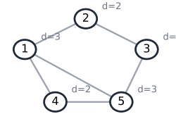
the picture (5 vertices, 6 edges)
