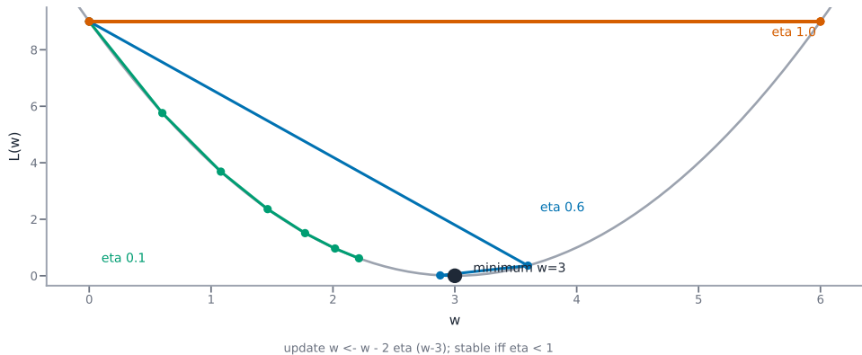
Contour ellipses around the minimum; three learning rates: small crawls, good descends, large overshoots
