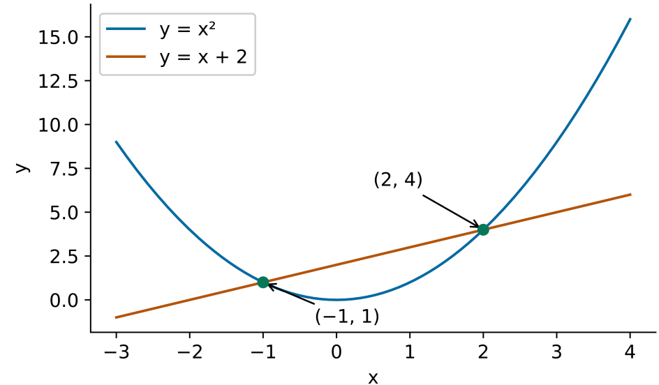
Two ordered pairs satisfy both relations
