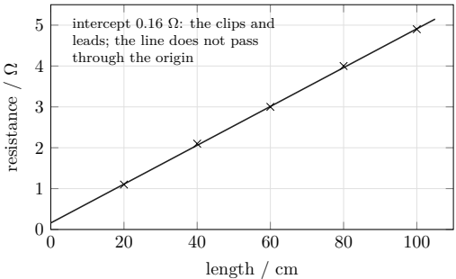
A straight line: resistance increases by the same amount for each extra 20 cm.
