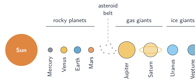
The Sun and its eight planets in order: four small rocky planets, then the asteroid belt, then four large gaseous planets — the gas giants Jupiter and Saturn and the ice giants Uranus and Neptune (not to scale)
