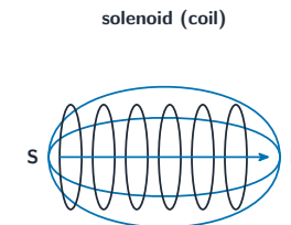
solenoid (coil) field like a bar magnet
