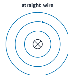
straight wire current into page; field is circles round it
