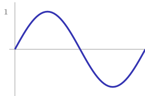
trig graphs
