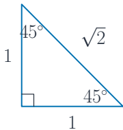
45^\circ triangle
