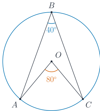
angle at centre = 2 \times angle at circumference
