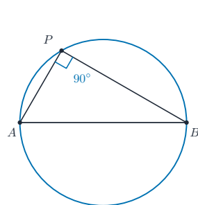
angle in a semicircle = 90^\circ
