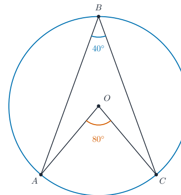
angle at centre = 2 \times angle at circumference
