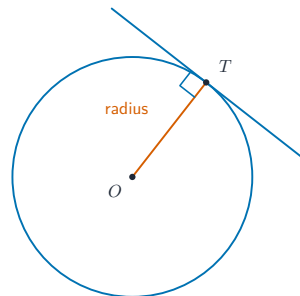
tangent meets radius = 90^\circ
