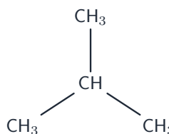
2-methylpropane (branched)
