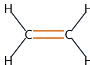
ethene C 2 H 4 unsaturated: C=C double bond
