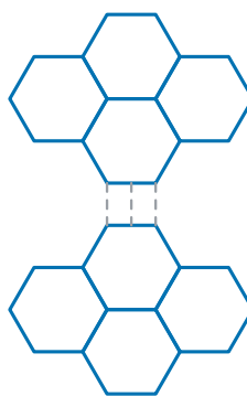
graphite
