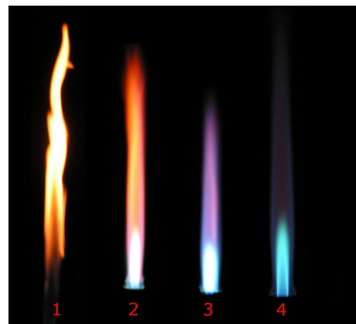
A Bunsen flame supplies energy: enthalpy change \Delta H is the heat transferred at constant pressure
