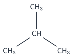
2-methylpropane (branched)
