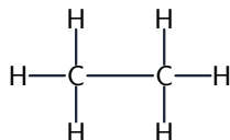
ethane C_2H_6 saturated: single C–C bond
