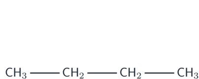
butane (straight chain)
