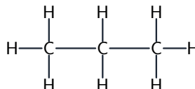
propane C 3 H 8
