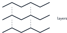
graphite (layers)
