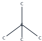
diamond (network)
