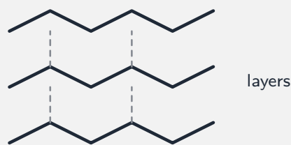
graphite (layers)
