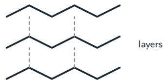
graphite (layers)
