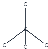
diamond (network)
