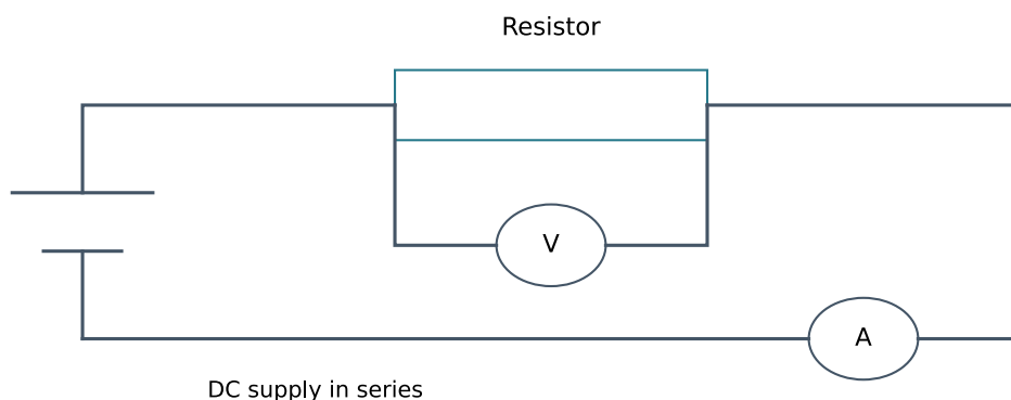
Ammeter in series; voltmeter across resistor
