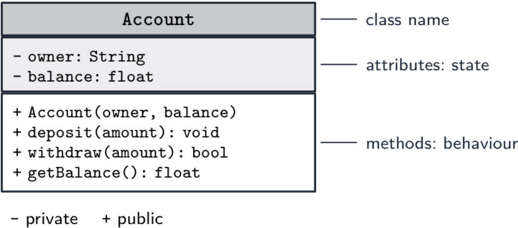
A UML class diagram: name, attributes, methods; - private, + public
