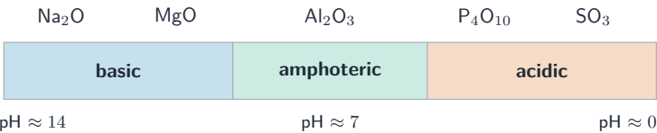
metal oxides (left) are basic; non-metal oxides (right) are acidic
