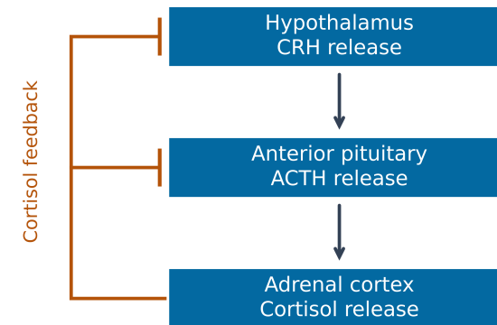
HPA axis: forward signals and feedback
