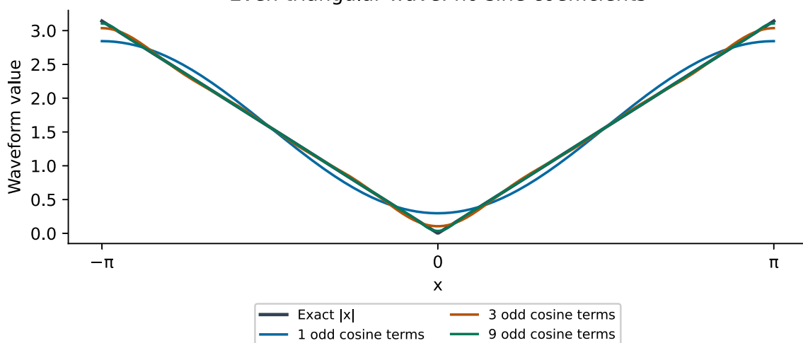
Even triangular wave: no sine coefficients
