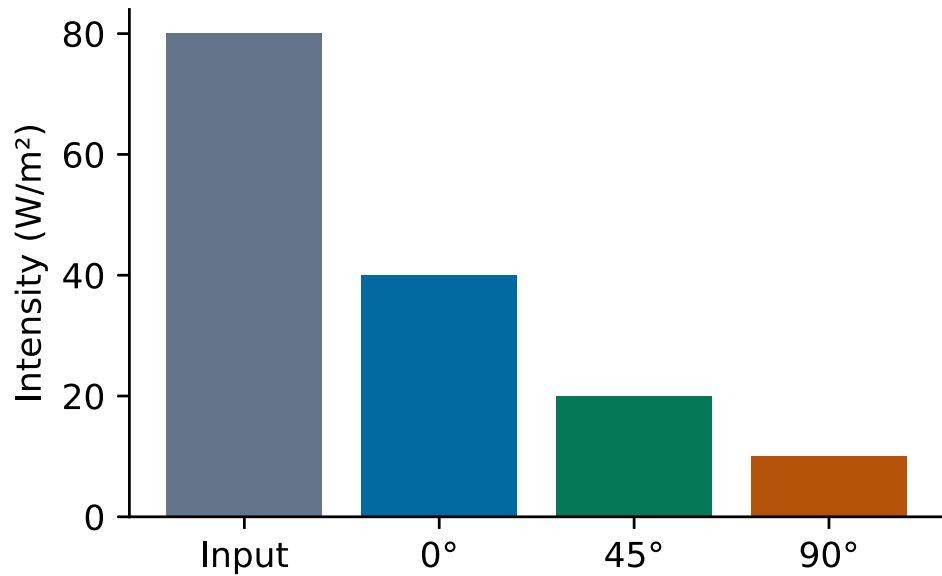
Unpolarised input; ideal analyser chain
