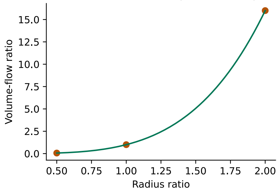
Laminar tube: fixed pressure drop
