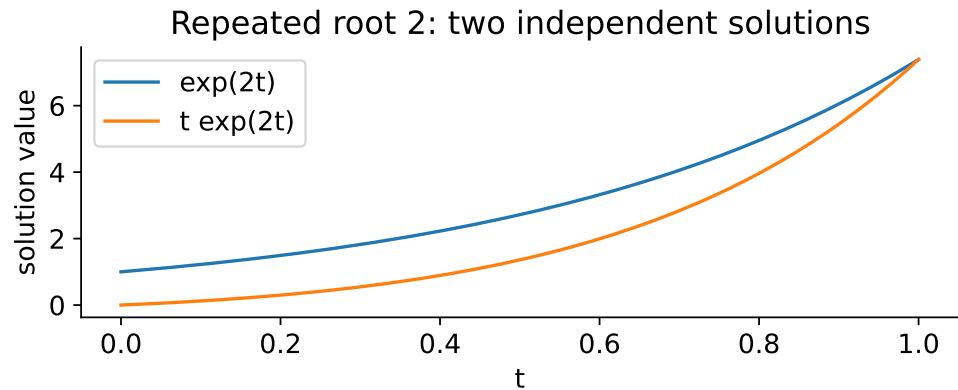
A repeated root 2 gives the two independent solutions e^{2t} and t \cdot e^{2t}
