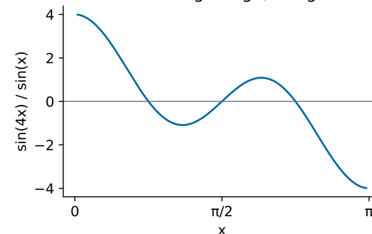
Reflection changes sign; integral zero
