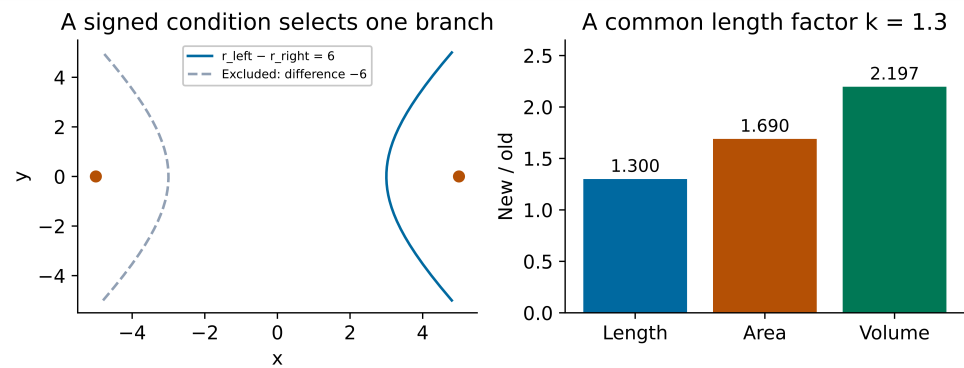
A signed difference picks one branch; a length factor k scales area by k^2 and volume by k^3
