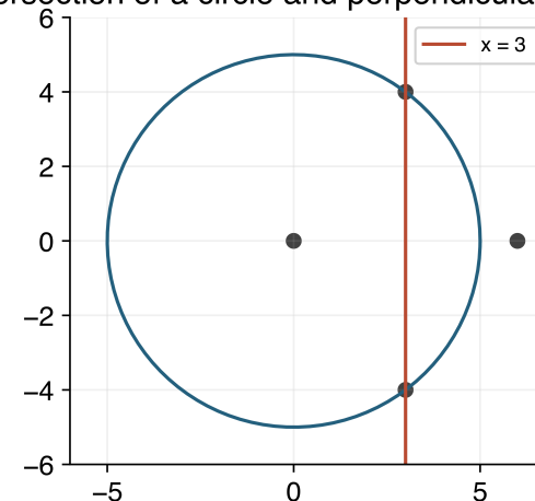
Intersection of a circle and perpendicular bisector
