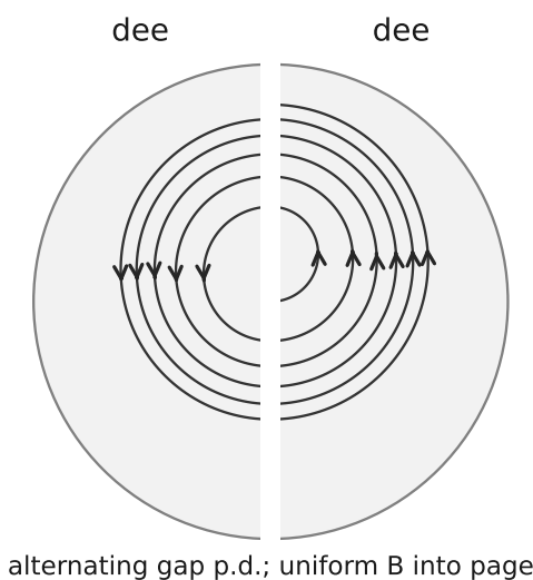
Cyclotron: radius grows after each gap
