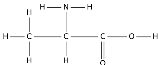
Displayed formula
