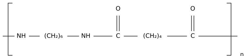
Condensation polymer repeat unit
