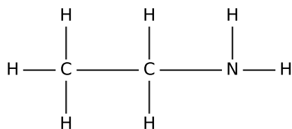
Displayed formula
