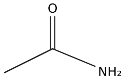
Skeletal formula
