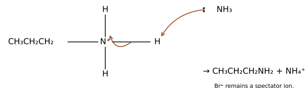
2 A second ammonia removes a proton
