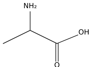
Skeletal formula
