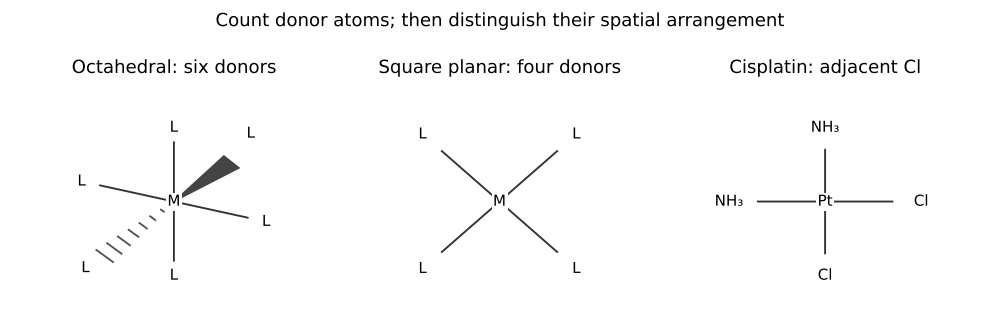
Six-coordinate octahedral and four-coordinate square-planar arrangements.
