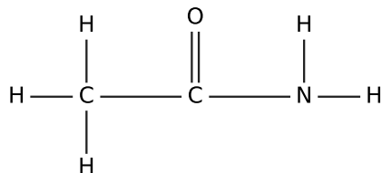
Displayed formula
