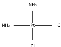
Cisplatin: adjacent Cl
