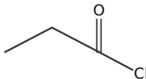
Skeletal formula
