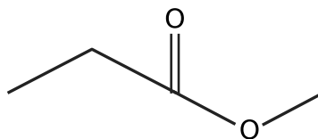
Skeletal formula
