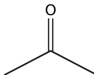
Skeletal formula
