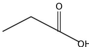
Skeletal formula
