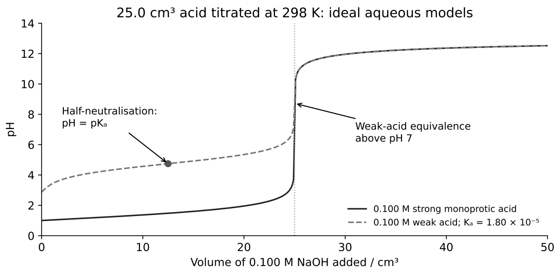
Strong and weak acid titration curves from ideal aqueous models.
