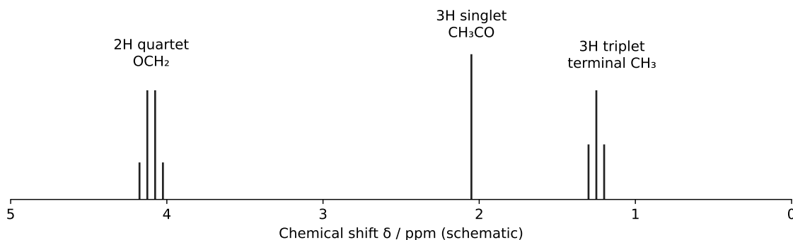
Schematic splitting and assignments for ethyl ethanoate.
