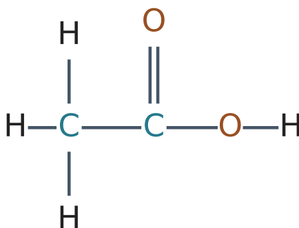
Ethanoic acid
