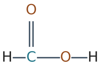
Methanoic acid
