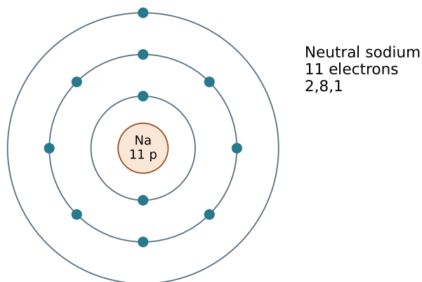
Energy-level model; distances and particle sizes not to scale
