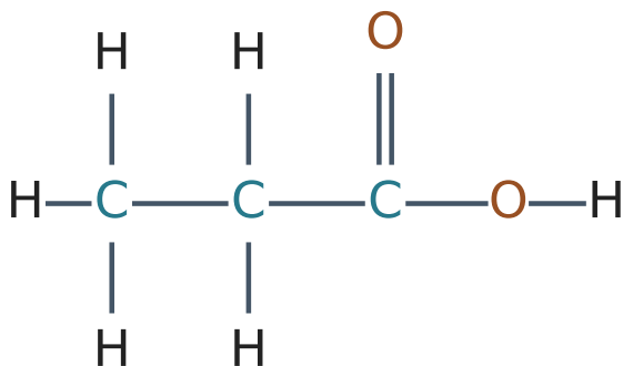
Propanoic acid
