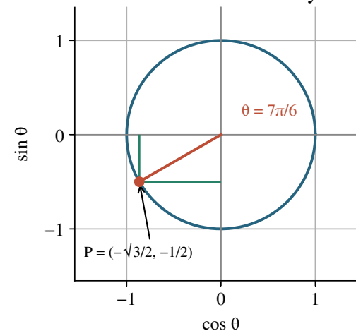
Coordinates define sine and cosine beyond acute angles
