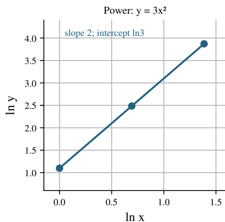
Different horizontal axes recover different parameters
