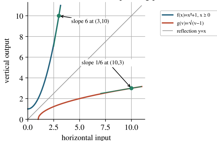
Inverse rates use reflected corresponding points
