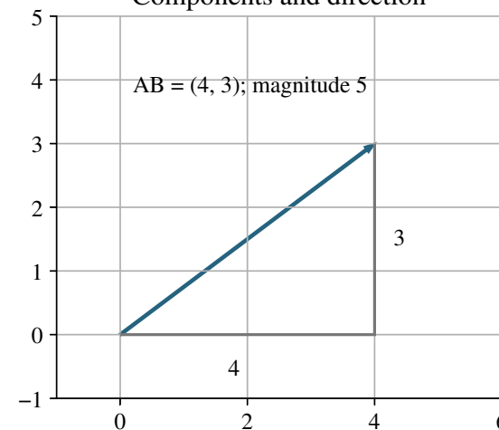
Components and direction
