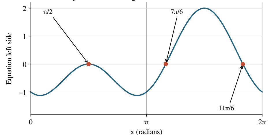
A quadratic in sine gives three roots in one turn
