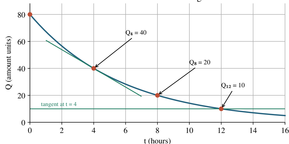
Fixed half-life: the absolute loss gets smaller
