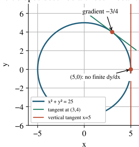
Implicit slopes describe a chosen local curve branch
