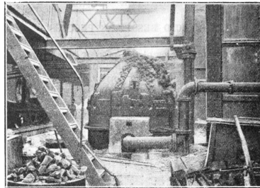
Fig. 30.—Bessemer Converter while Blowing.
