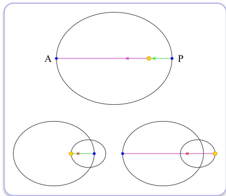
An orbit traced as x(t) , y(t)
