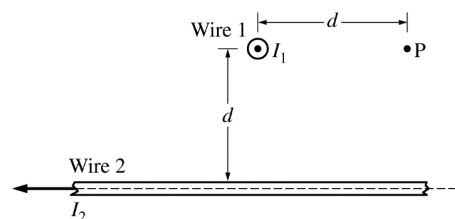
Figure 1. Side view
