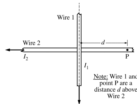
Figure 2. Top view
