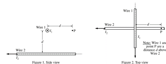
Figure 2. Top view
