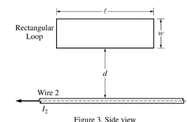
Figure 3. Side view
