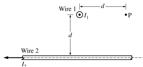
Figure 1. Side view
