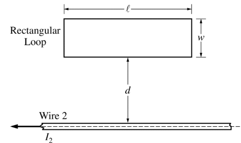
Figure 3. Side view
