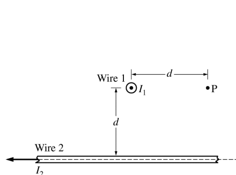
Figure 1. Side view
