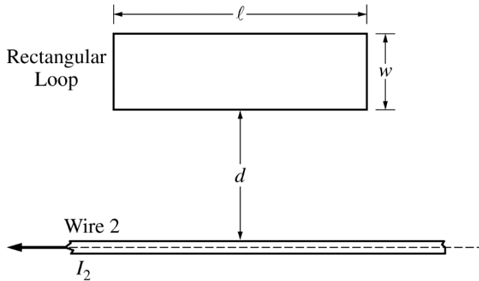
Figure 3. Side view
