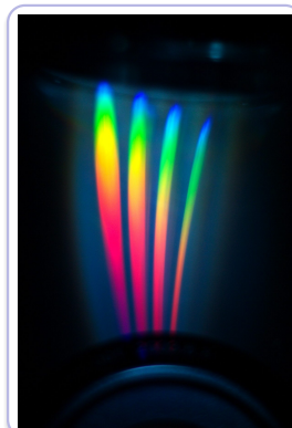
Diffraction reveals the wave nature of light
