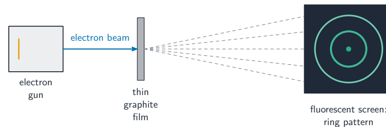
Electrons form a diffraction pattern, showing that particles have a wave nature
