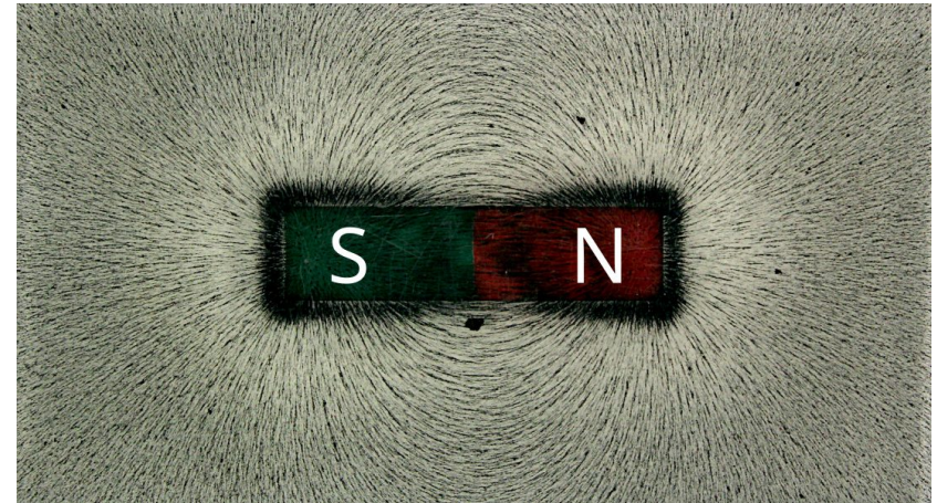
Iron filings line up along the magnetic field, making the invisible field lines of a bar magnet visible
