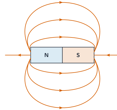
Field lines run from N to S outside a bar magnet, closer where the field is stronger
