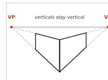
Two-point perspective
