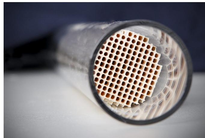
A catalytic converter: catalysts speed rates by lowering activation energy without being consumed
