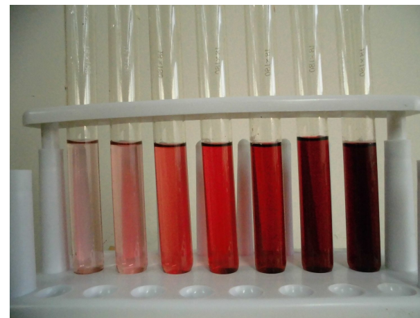
Cobalt chloride solutions: equilibrium systems shift when conditions change (Le Chatelier)
