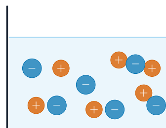
strong acid
