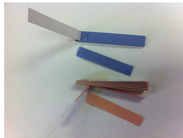
Litmus paper: acid–base indicators change colour with H^+ concentration (pH)
