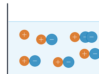
weak acid
