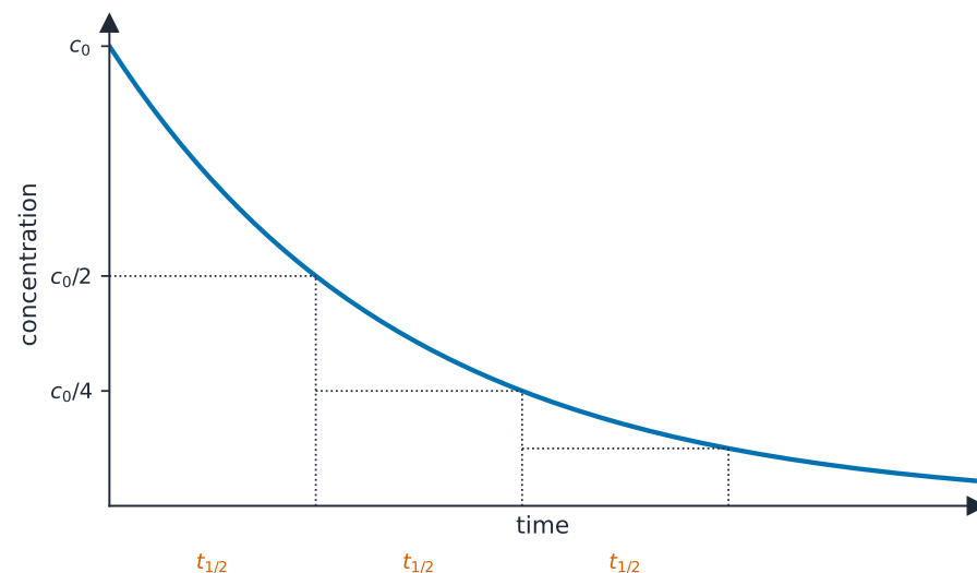
A first-order reaction has a constant half-life
