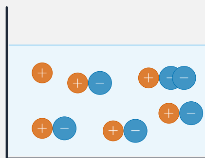
weak acid mostly molecules: few ions
