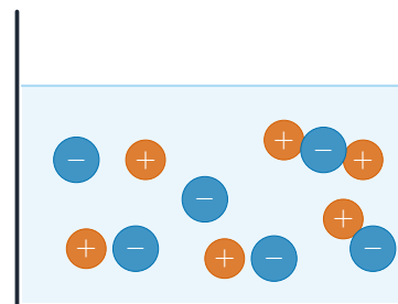
strong acid fully dissociated: many ions
