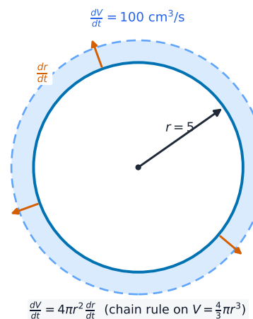
An inflating balloon links dV/dt and dr/dt through the chain rule
