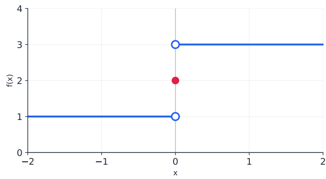
One-sided heights 1 and 3 at 0, with a separate filled point at height 2.
