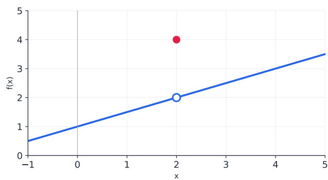
A curve with an open point at (2,2) and a filled point at (2,4).
