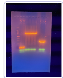
Gels sort DNA; PCR amplifies a target
