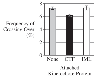
Figure 2. The frequency of crossing over in a hotspot on yeast chromosome 8 for cell groups treated with different kinetochore proteins. Error bars represent \pm 2SE .
